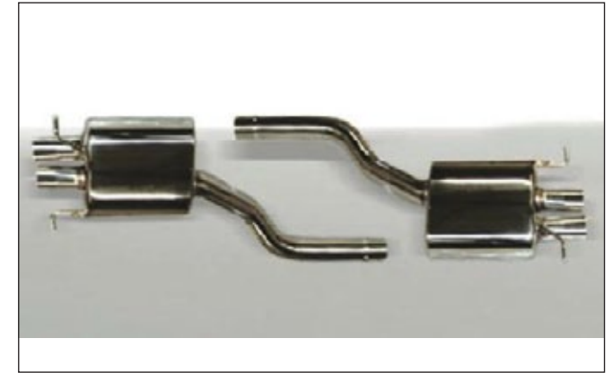
Sport mufflers W12 ..... 630 253 615 Sport mufflers V8 ..... 630 253 616
