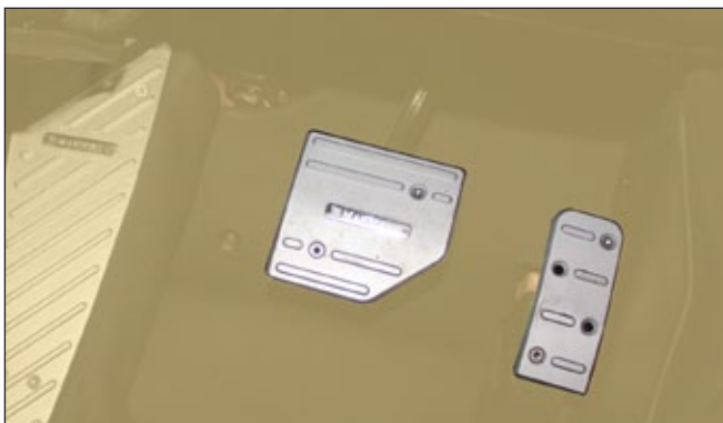
Pedal pads, LHD 458 400 15 2 parts set Consisting acceleration & brake pedal made of anodized aluminium.
